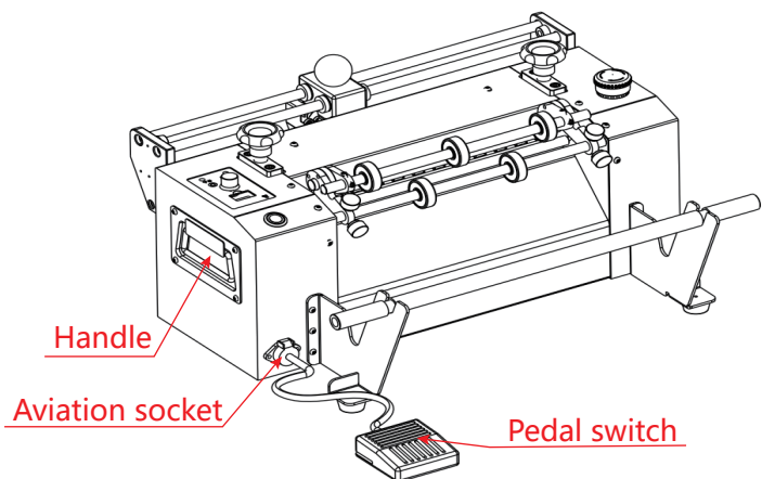
Figure 2 (Full view of the machine)
